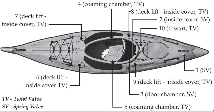
Diagram of Inflation Chambers
