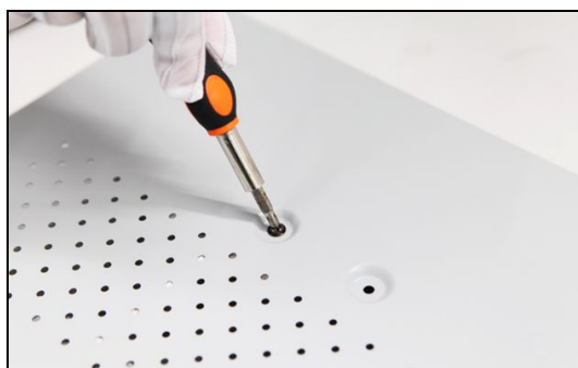
Figure 2. 4 Install the HDD
