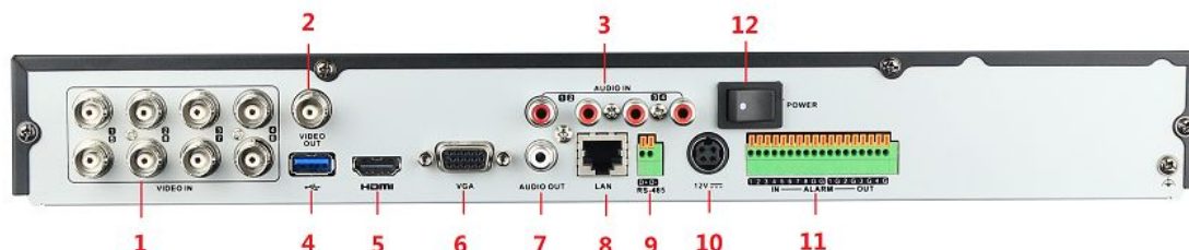
Figure 1. 2 Rear Panel
