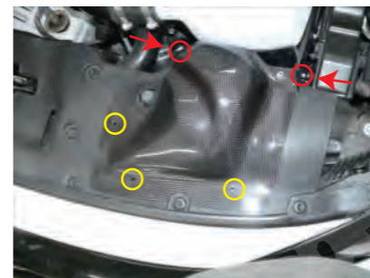
31. Attach the front introduction duct. Red : Bolt D Yellow : Clip
