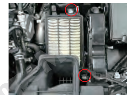
3. Take out the lower part of the box by removing the 2 bolts holding it in place.
