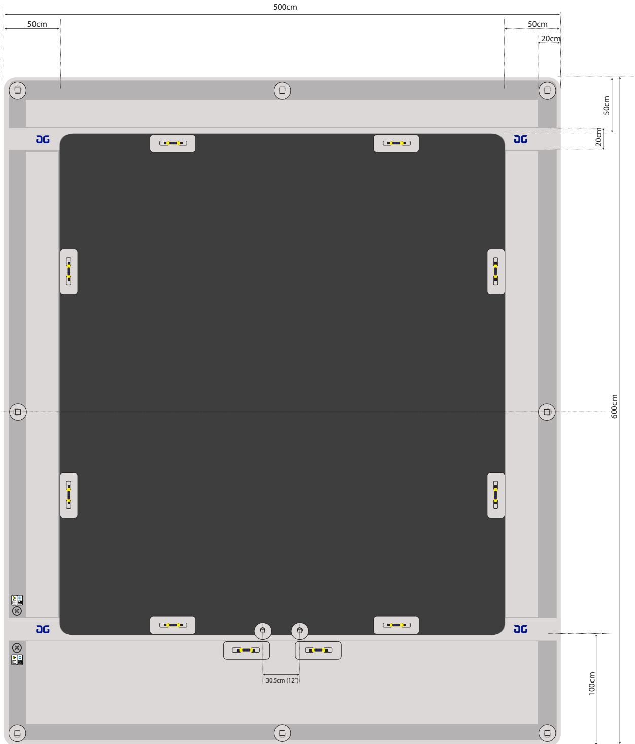
TOP VIEW
