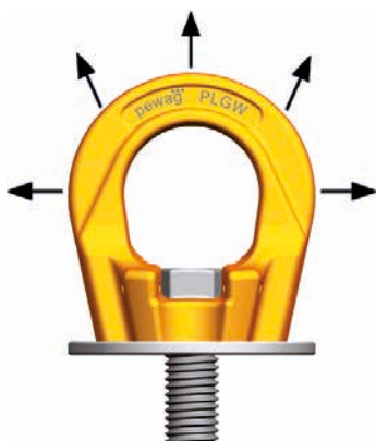
Permissible pull directions that occur when used correctly.
