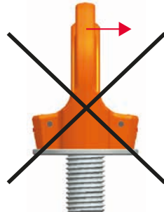
Non-permitted directions of pull
