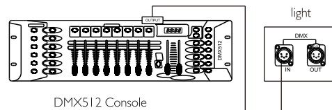
DMX connection for single light
