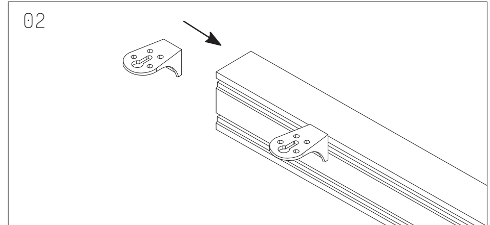
Join 1 L-Bracket through each 1295mm Beam and 1 L-Bracket through each 295mm Beam.
