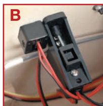
Kwik-Switch Mount & Charging Jack Inside view
