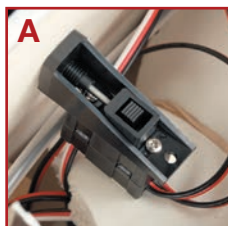
A Kwik-Switch Mount & Charging Jack Inside view
