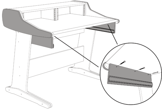
10 M5x50
