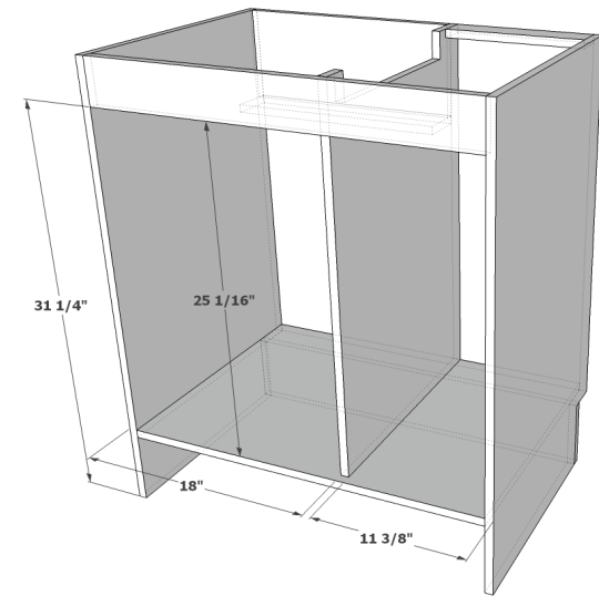
BACK DETAIL
