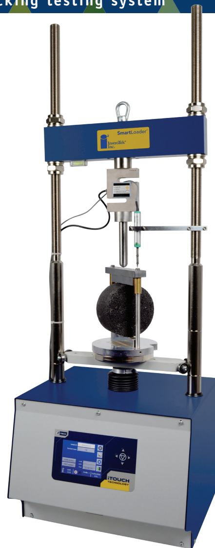
IDEAL-CT configuration
