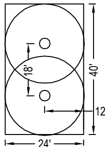
TYPICAL COVERAGE TWO HEATERS
