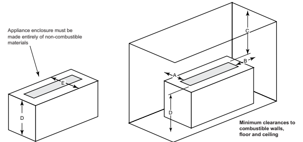
CLEARANCES
