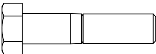
(A3)HEX BOLT 1/2"X2-1/4"L PARTIAL QTY.2
