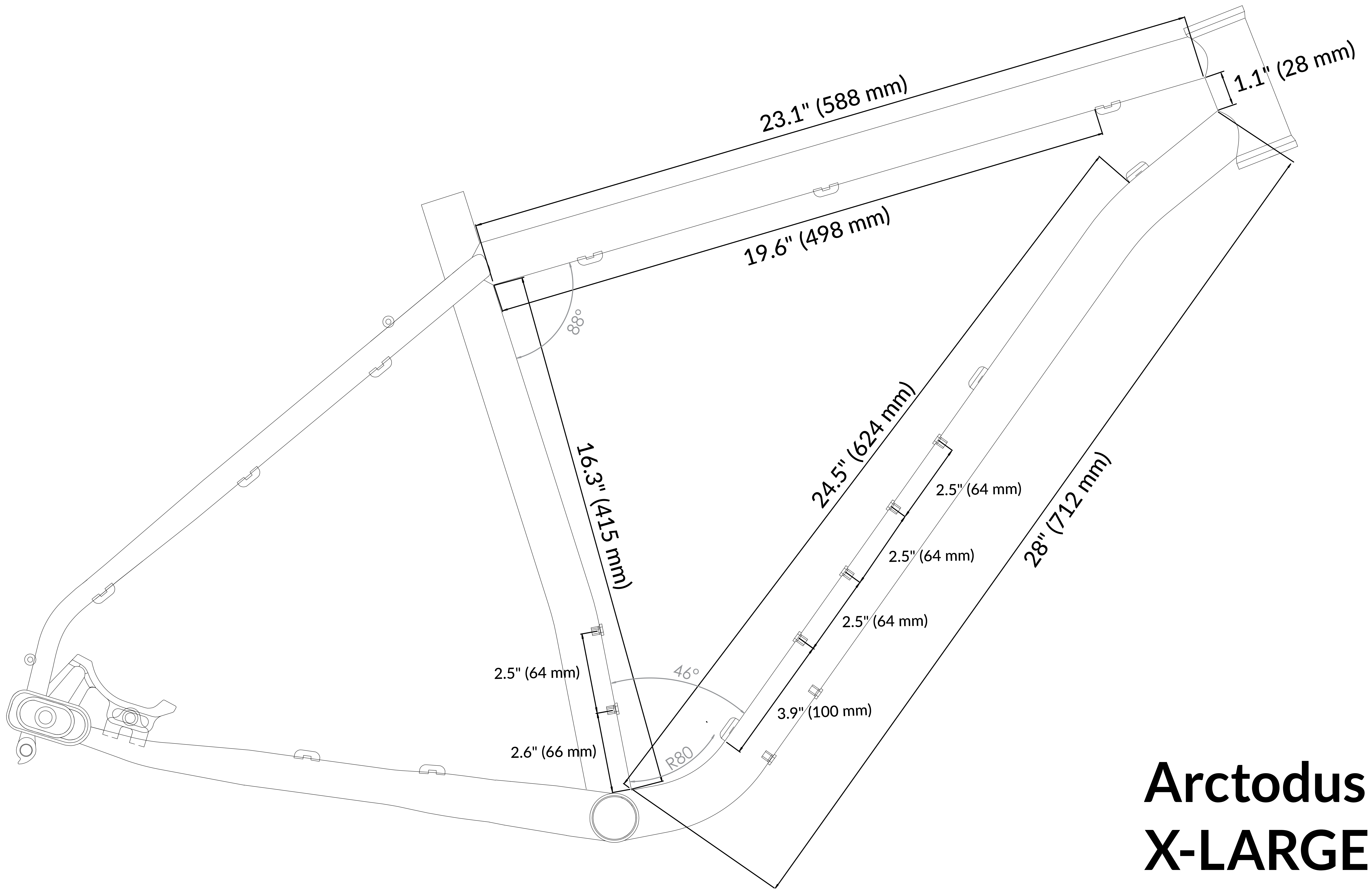
Frame Bag Dimensions
