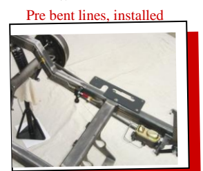
Brake System
