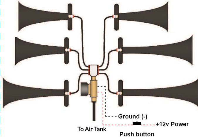
Option 1: Honk with push button
