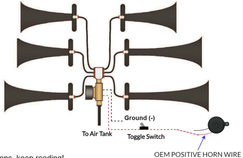
Option 2: Honk with Steering Wheel
