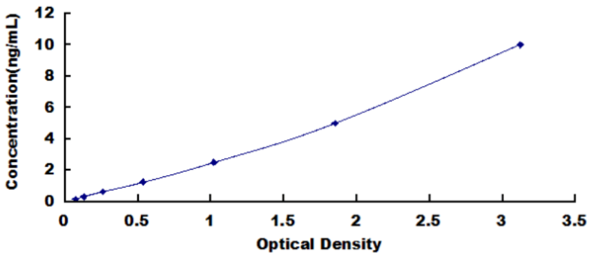
Typical Standard Curve for Rat GAP43 ELISA
