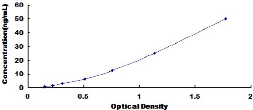
Typical Standard Curve for Rat CALU ELISA
