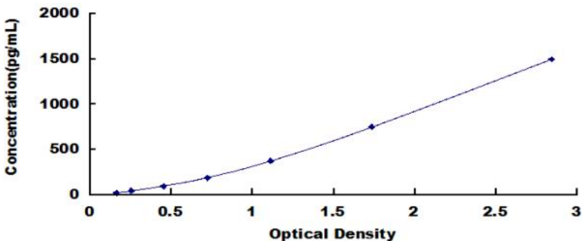
Typical Standard Curve for Rat MDC ELISA
