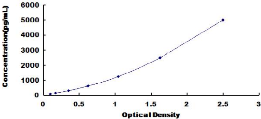
Typical Standard Curve for Rat FGF10 ELISA
