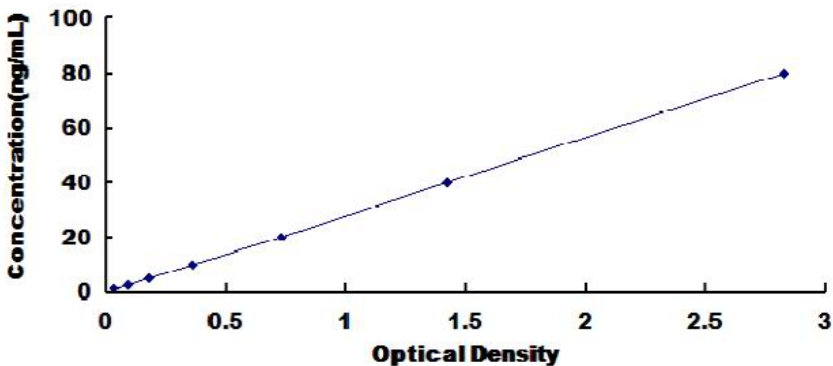
Typical Standard Curve for Porcine MSTN ELISA
