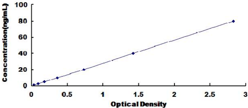
Typical Standard Curve for Mouse aZGP1 ELISA
