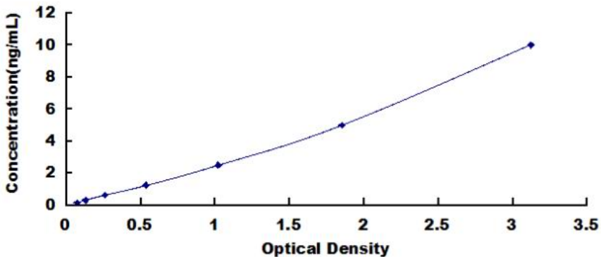
Typical Standard Curve for Mouse FGFR1 ELISA
