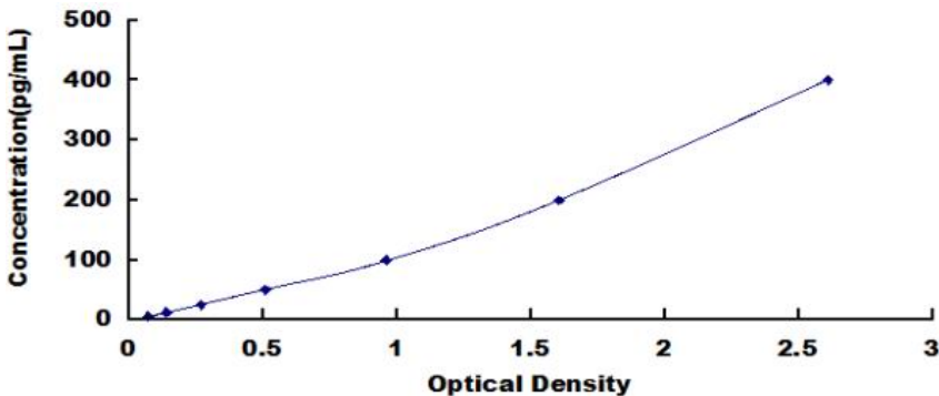
Typical Standard Curve for Human PLA2G2A ELISA
