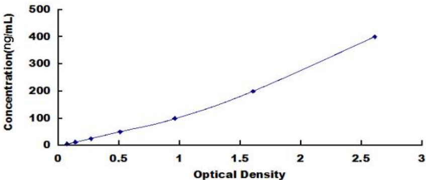
Typical Standard Curve for Human GPX3 ELISA
