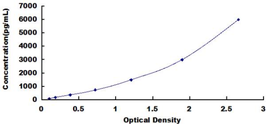
Typical Standard Curve for Human ENPP2 ELISA
