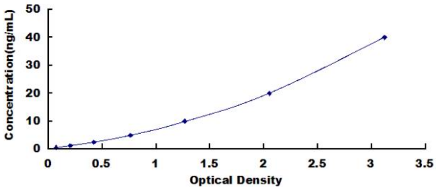
Typical Standard Curve for Human BAK1 ELISA
