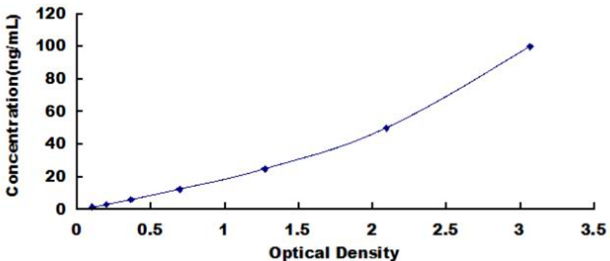
Typical Standard Curve for Human ASS1 ELISA
