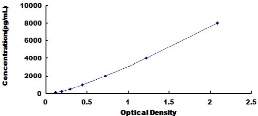
Typical Standard Curve for Human MYL1 ELISA
