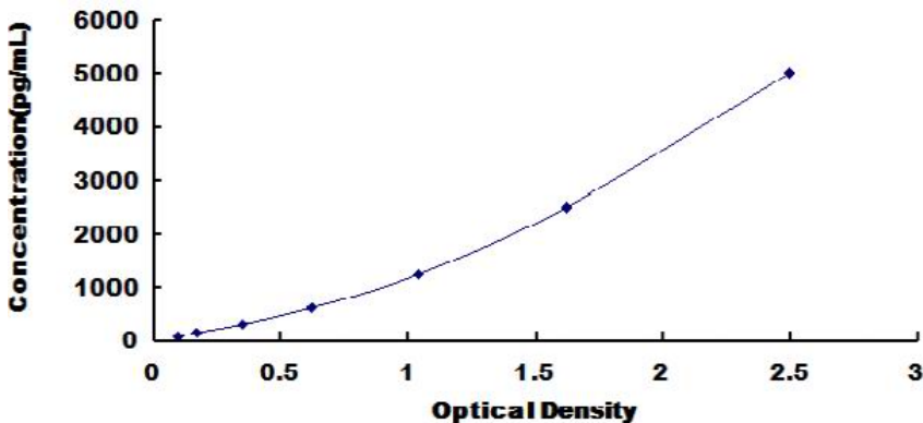
Typical Standard Curve for Human GPC1 ELISA
