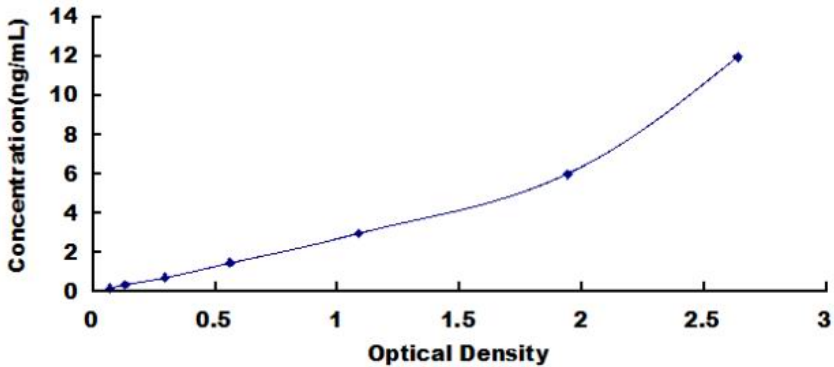
Typical Standard Curve for Human ANGPTL3 ELISA
