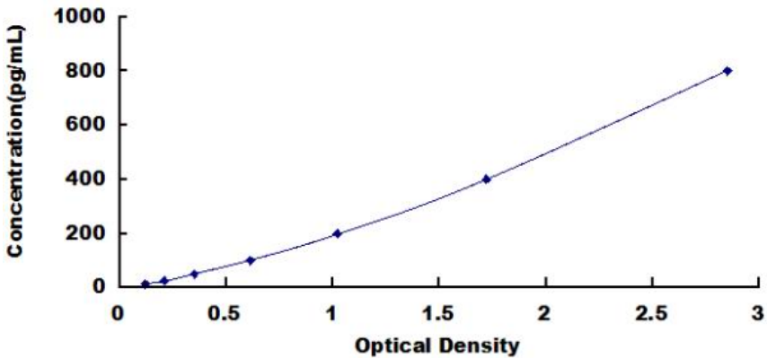
Typical Standard Curve for Human PAI1 ELISA
