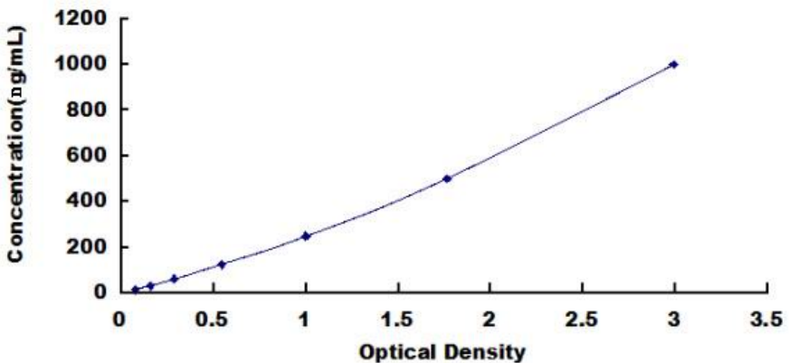
Typical Standard Curve for Bovine a2PI ELISA
