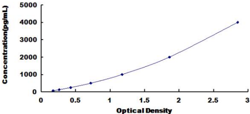
Typical Standard Curve for Bovine IGFBP3 ELISA
