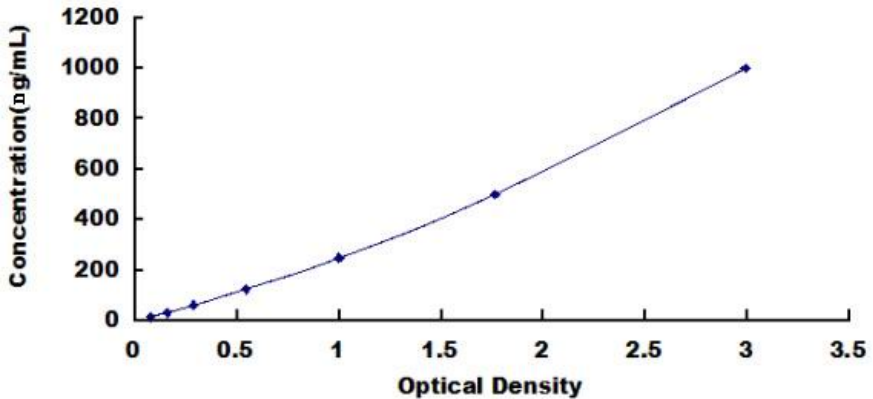
Typical Standard Curve for Monkey IL1b ELISA
