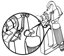
G-08/10 locked off (gun will not spray)
