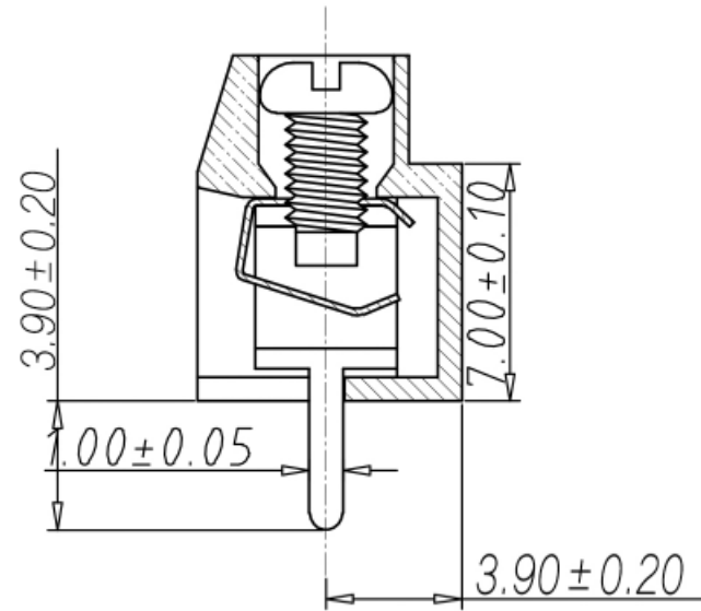
Sectional View A-A
