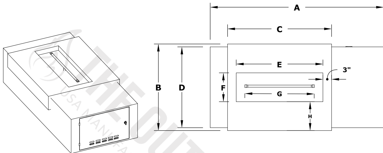
ISOMETRIC VIEW
