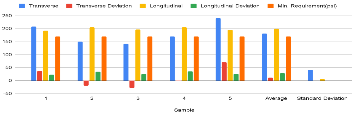
Breaking Strength ASTM D751-06(2011)
