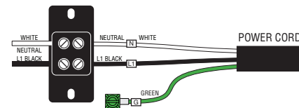
200V 2 WIRE + GROUND
