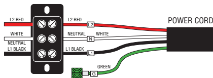
120/208-240V 3 WIRE + GROUND
