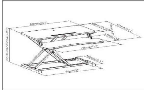
Product Drawing
