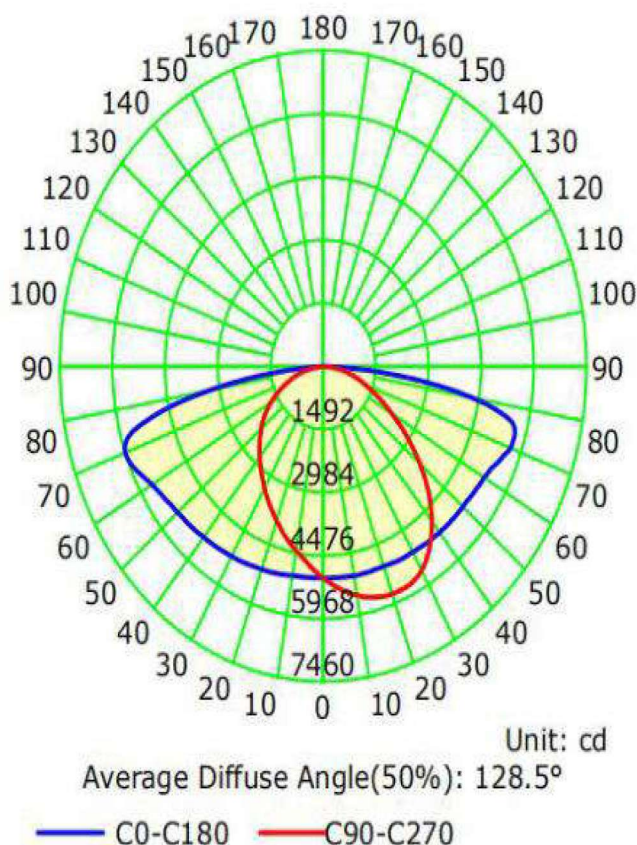
Luminous Intensity Distribution Curve
