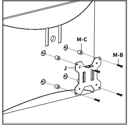
Side VESA Plate (J) Installation
