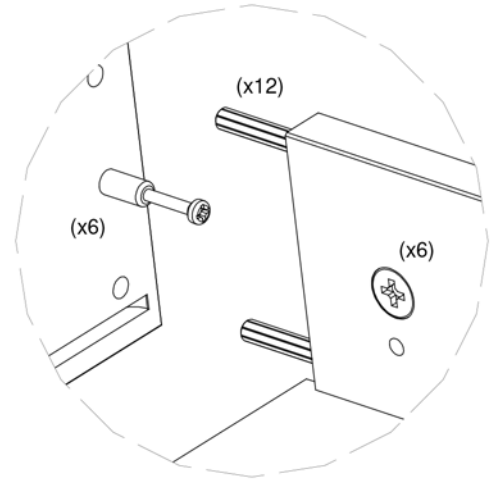
Detail F
