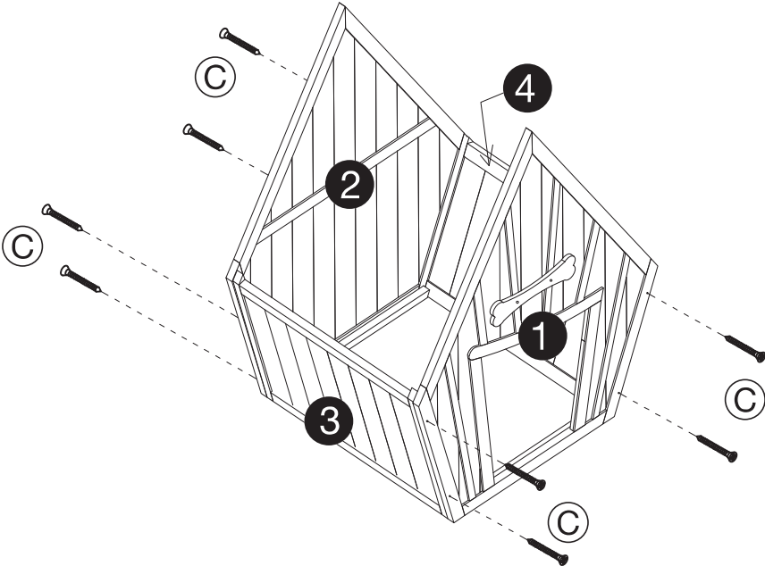
STEP 1 CONNECT WALL PANELS
