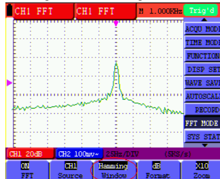
Figure 58: Hamming window
