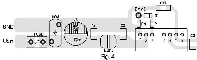
Note: the min. distance of the bonding pads between input grounding and output grounding shall be \geq 2\text{mm} .
