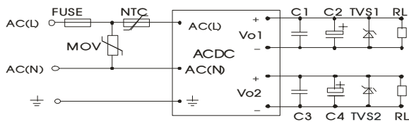
Fig. 3: LH20-10D series (Isolate Twin Output) typical application circuit
